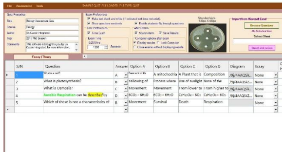
Fig 2. Objective questions input screen
